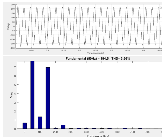
Figure 9: Voltage waveform and FFT analysis ANN based Multilevel converter
