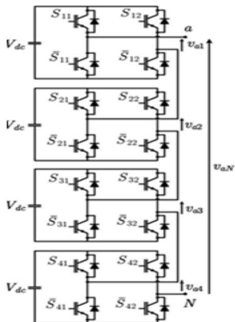
Figure 1: connection schematic of a single phase cascaded H- bridge Nine level Inverter
