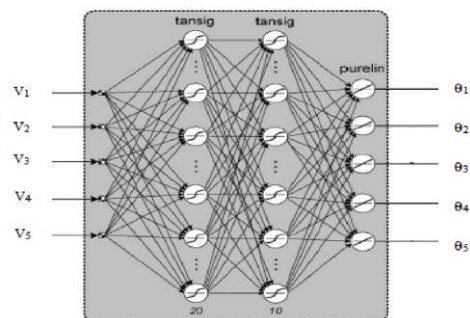
Figure 3: Neural Network structure
