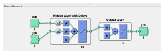
Figure 3: Neural Network structure
