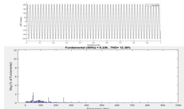
Figure 7: Voltage waveform and FFT Analysis for Output Voltage Waveform (PI controller)
