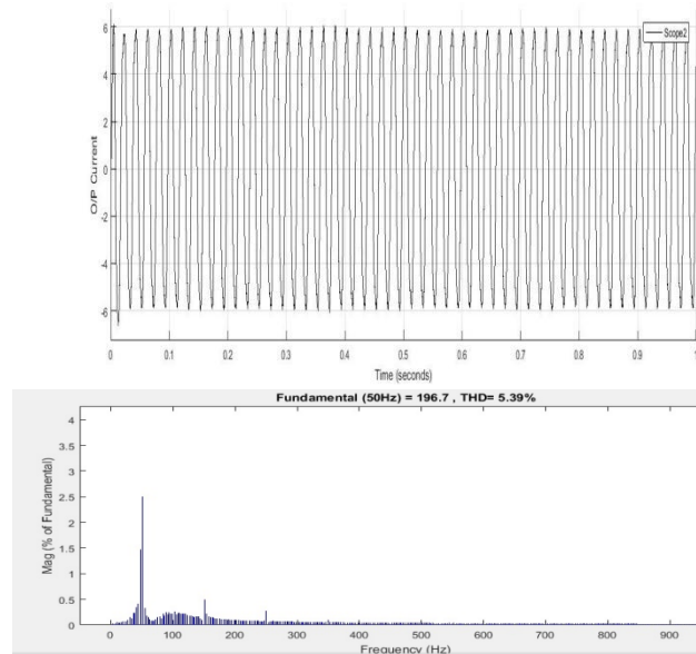
Figure 8: Current waveform and FFT Analysis for Output Current Waveform (PI Controller)
