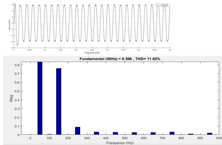
Figure 10: Current waveform and FFT analysis ANN based Multilevel converter PWM block has the facility to determine the modulation index which is the ratio of peak of modulating signal to peak of the carrier signal. With this block, amplitude frequency and phase delay is adjusted. The shape of the output voltage waveform is decided by selecting the parameters of the PWM block. Ripples are reduced and efficiency of the DC to AC conversion is increased. In Multilevel converter it is possible to deliver very high voltage and good quality of power with less harmonics with the help of Neural Network. The resistive-inductive loads are connected across the cascaded H-bridge nine level inverter. Output voltage remains constant to the reference value. The total harmonic distortion is 5.39%. The total harmonic distortion in current waveform is 12.23% with the PI controller whereas with the help of ANN. The THD content in voltage and current waveform is reduced to 11.65% and 3.66% respectively.
