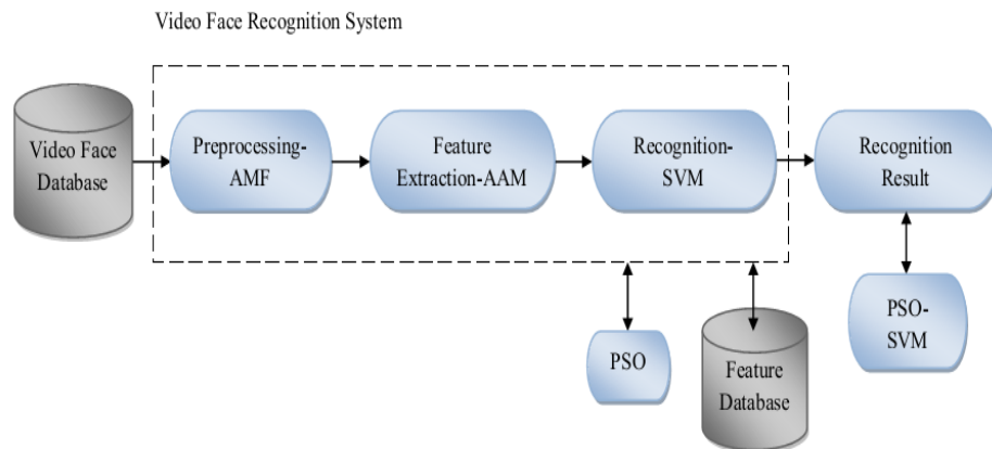
Figure 1: Structure of our proposed video face recognition system based on PSO-SVM
