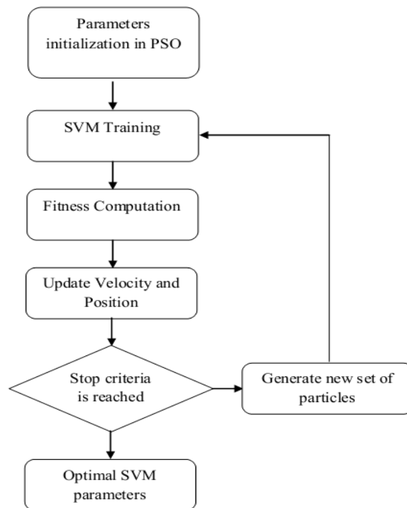
Figure 2: SVM parameters optimization by PSO
