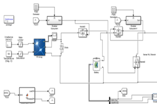
Fig.4 Simulink Model of Proposed charge controller
