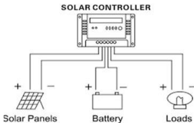
Fig.1 Block Diagram of Solar Charge Controller Connection
