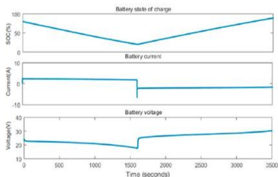
Fig.5 Output Waveforms of combined series and shunt charge controller
