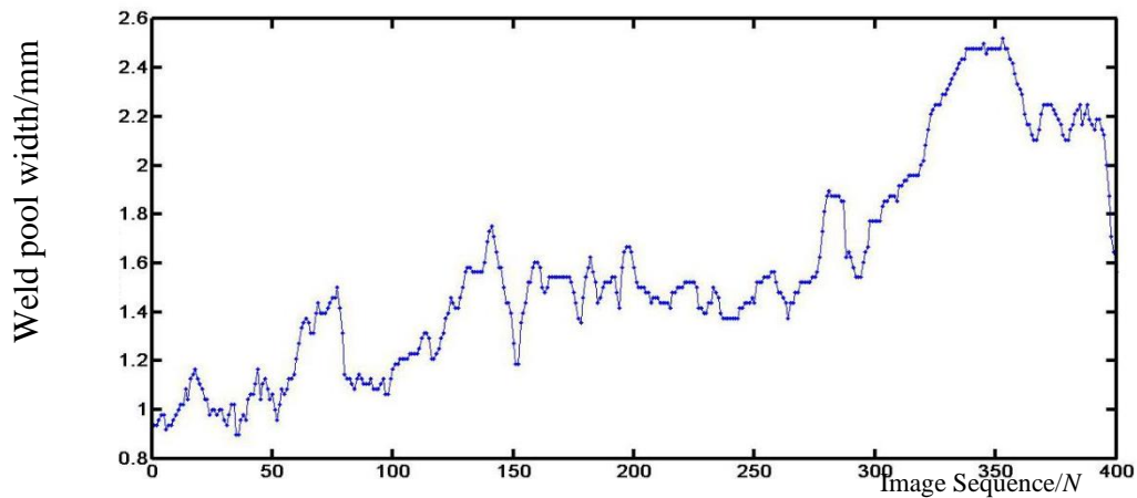
Fig.7. Weld Pool Width at the Back of Weld Seam
