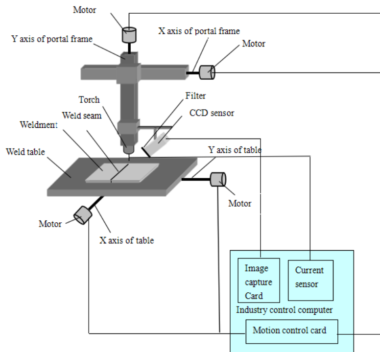
Fig.1. Welding Experimental System
